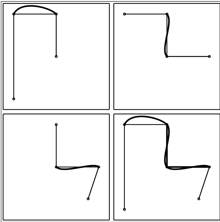
Figure 5.4: Overhauser curves
